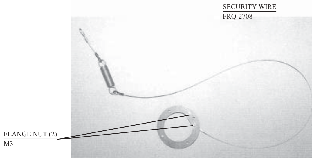
PHOTO 10. 1 e Security Plate (Reverse)
