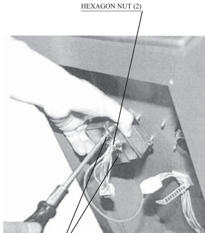
SCREW (2) M4 X 8,w/flat & spring washers
